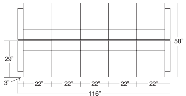
Back-To-Back Configuration using 10 1-Seat Modules with 4 Outside Arms
